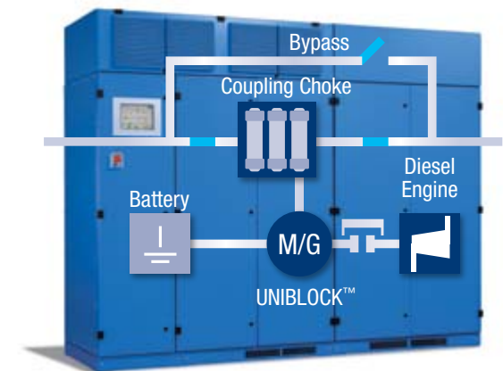
UBTD+ with external battery ride-through.
