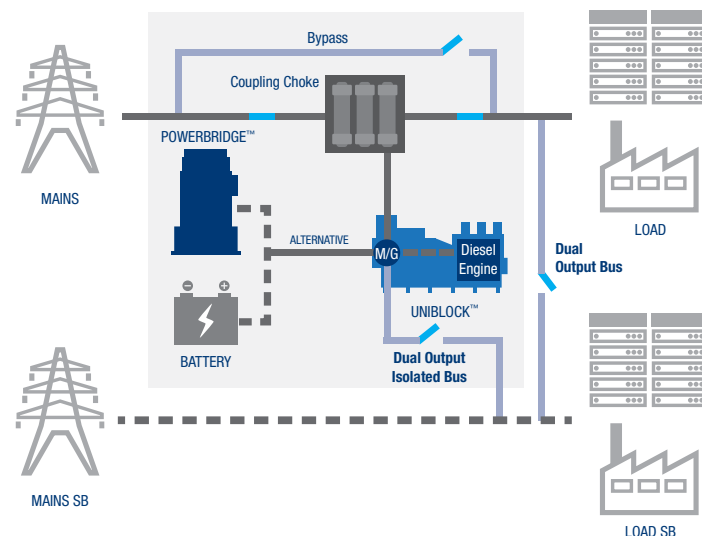
UNIBLOCK™ UBT+ with alternative Dual Output Bus configurations.
