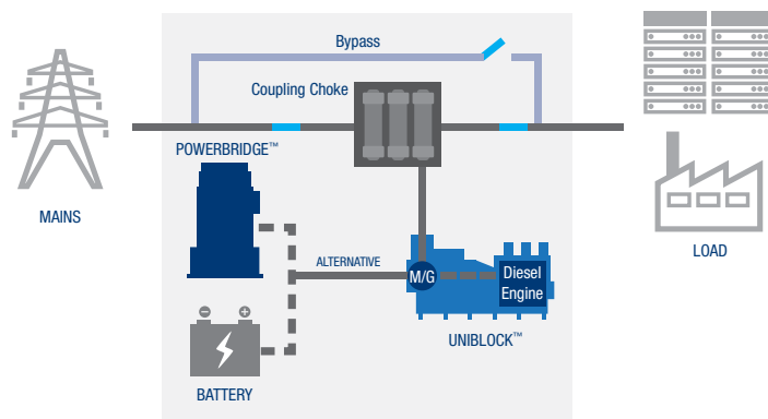
UNIBLOCK™ UBT+ in standard output configuration.
