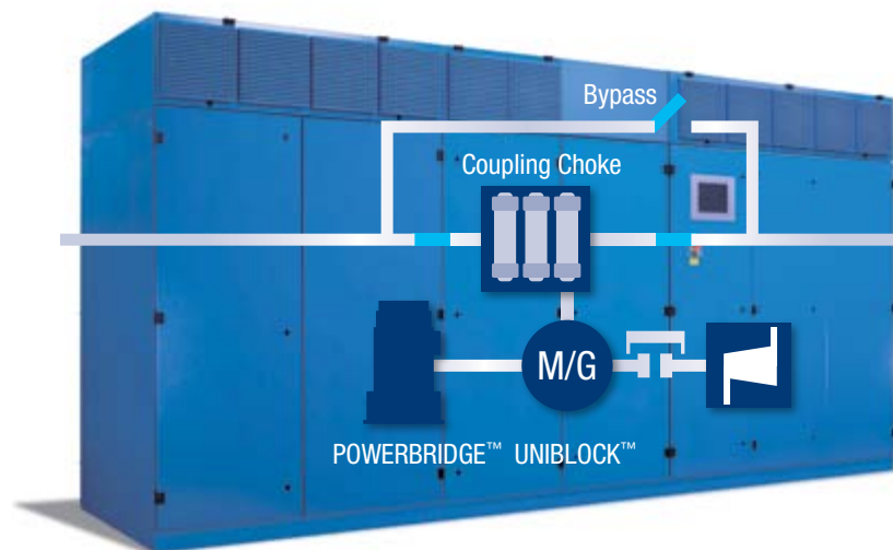
UBTD+ with POWERBRIDGE™ kinetic energy store.
